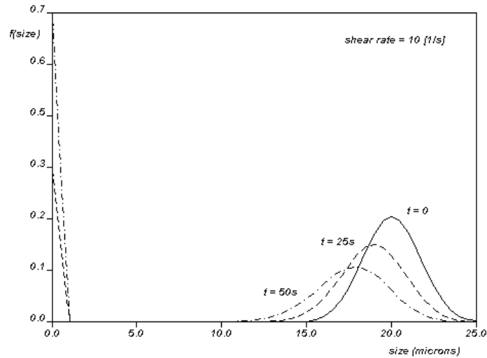
Effect of erosion on the mass distribution function as a function of time; the matrix viscosity is 11000 Pa.s and the shear rate is 10 s -1 .
