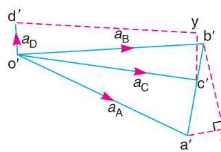
(c) Acceleration diagram.
