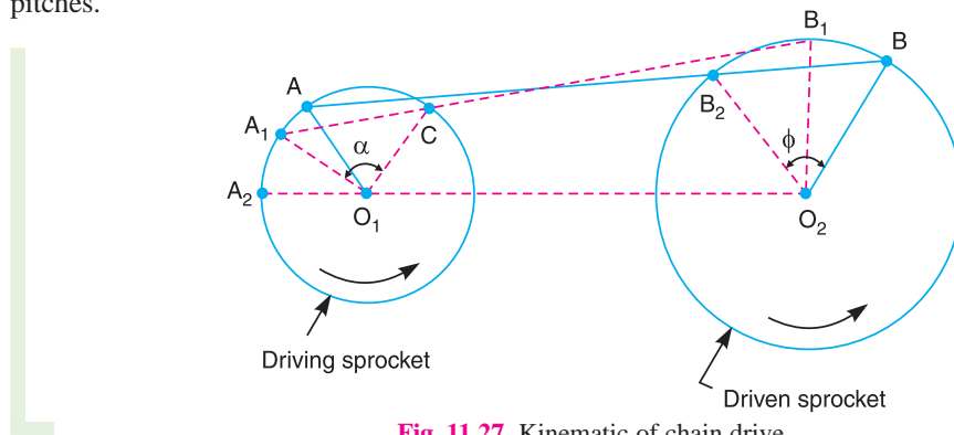
Fig. 11.27. Kinematic of chain drive.
