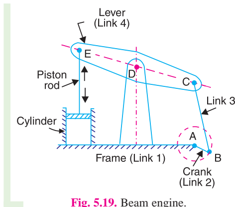
Fig. 5.19. Beam engine.
