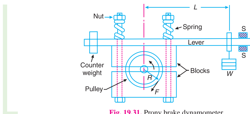
Fig. 19.31. Prony brake dynamometer.
