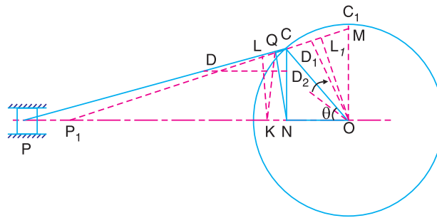
Fig. 15.4. Bennett's construction.
