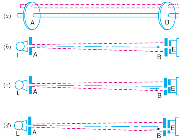
Fig. 19.36. Bevis-Gibson flash light torsion dynamometer.
