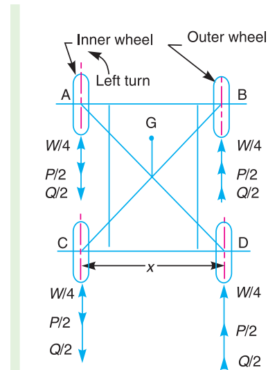
Fig. 14.11. Four wheel drive moving in a curved path.
