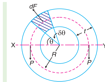
Fig. 16.17. Rim of a flywheel.
