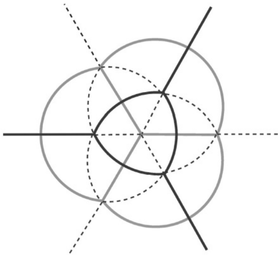
FIG. 131: TETRAHEDRON–TETRAHEDRON
