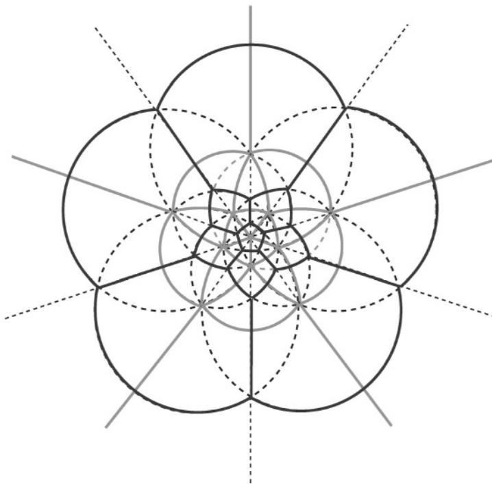
FIG. 133: DODECAHEDRON-ICOSAHEDRON
