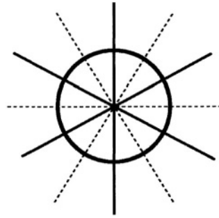
FIG. 130: 6-DIHEDRON
