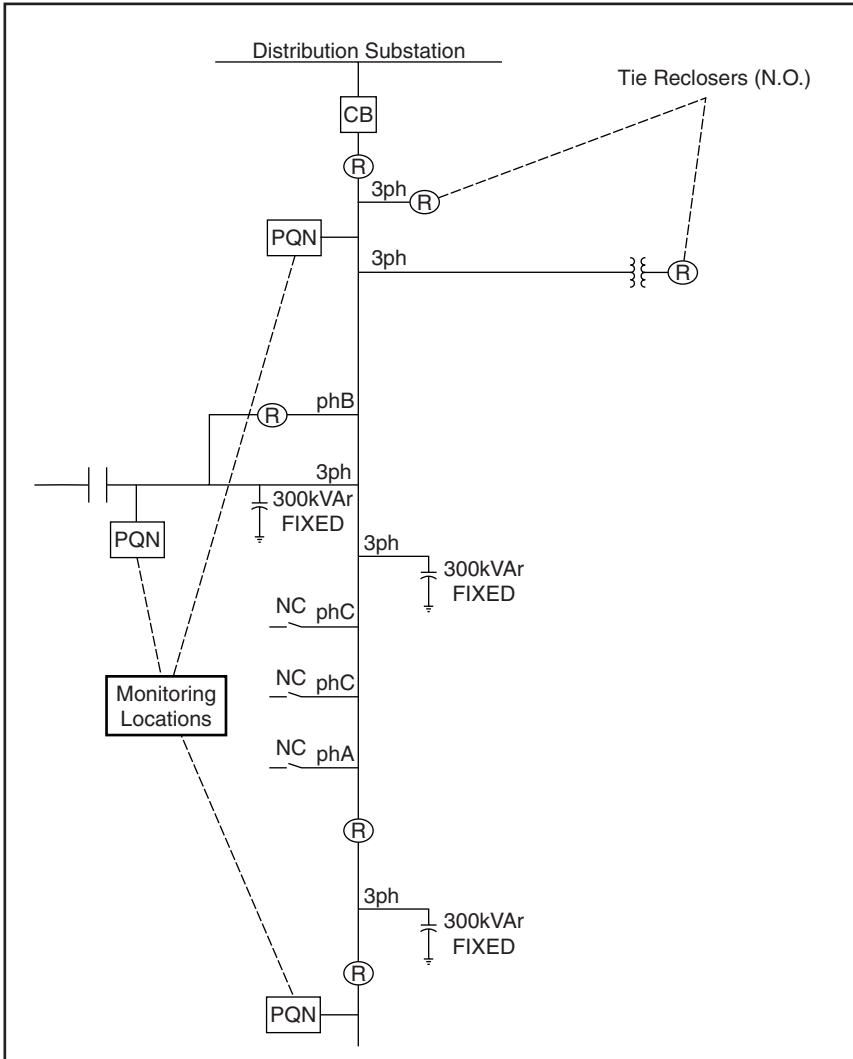
Figure 11.5 Typical distribution feeder monitoring scheme.
