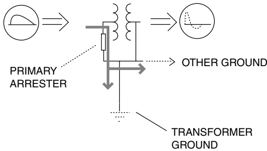
Figure 4.8 Lightning impulse bypassing the service transformer through ground connections.
