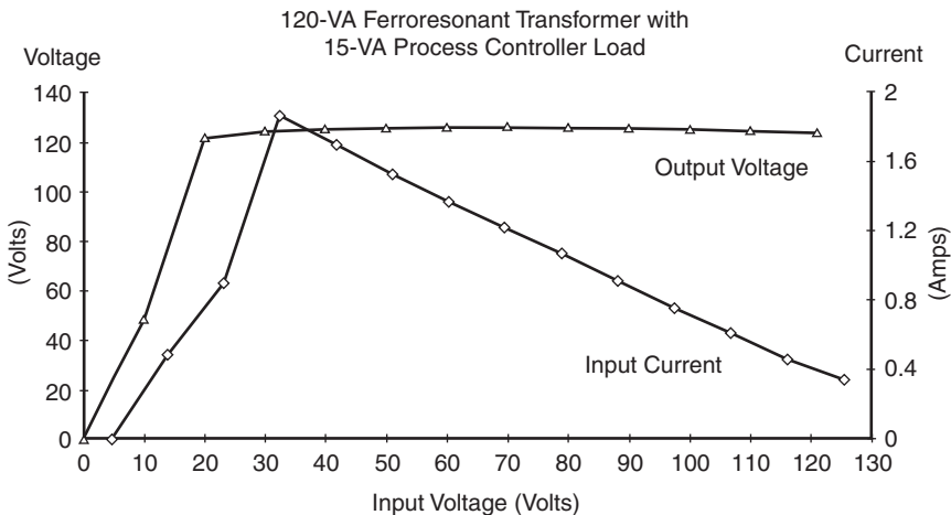
Figure 7.3 Ferroresonant transformer steady-state characteristics.
