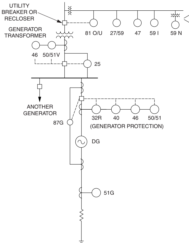
Figure 9.37 Protection scheme for a large synchronous generator with high-side recloser.
