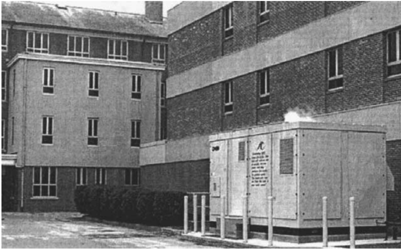
Figure 9.5 A fuel cell producing electricity and heat for a hospital. (Courtesy of International Fuel Cells, LLC.)
