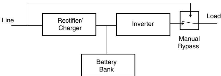
Figure 3.21 On-line UPS.
