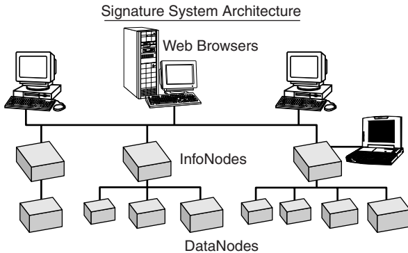
Figure 11.20 A smart power quality monitoring system—it turns data into information on the spot and makes it available over the Internet. (Courtesy of Dranetz-BMI.)
