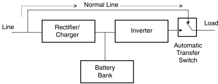
Figure 3.22 Standby UPS.
