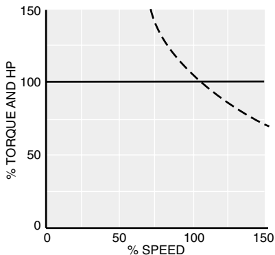
Figure 8.7, Constant Horsepower
