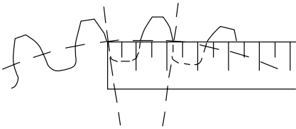
Figure 4.2, Worm Gear
