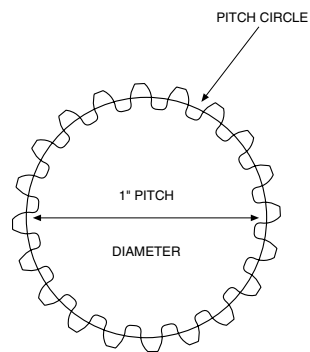
Figure 2.2B, A gear with 20 teeth and a 1" Pitch Diameter is 20 Pitch.
