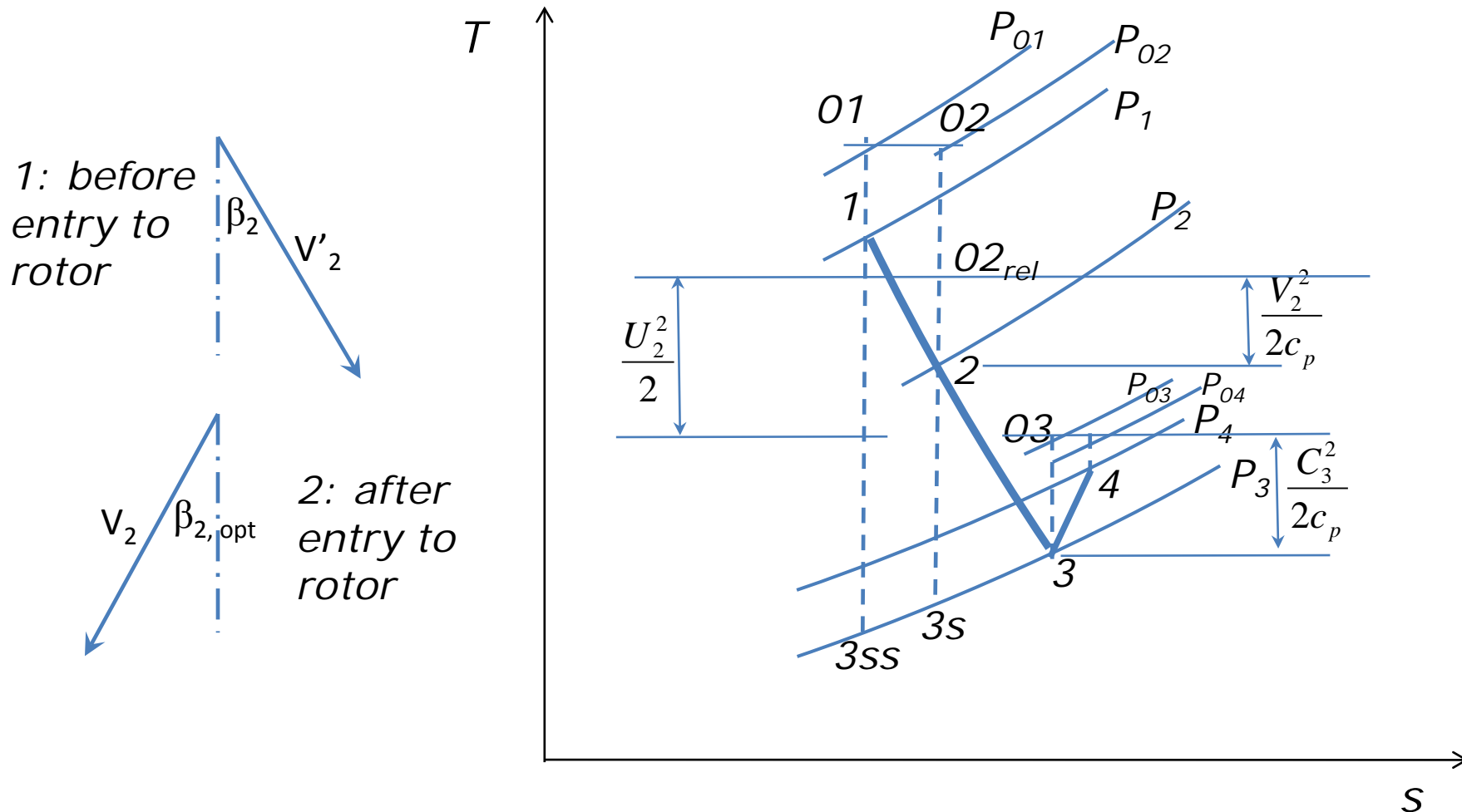
T-s diagram for an IFR turbine
