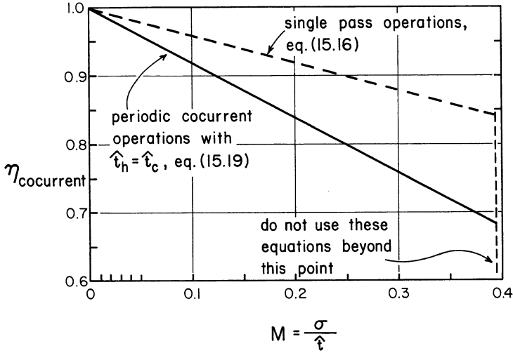
Fig. 15.10 Periodic cocurrent operations always lead to a lower efficiency than do single-pass operations. Both curves are drawn for a switching time of \hat{\tau} and are based on the dispersion model
