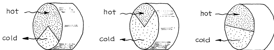
Fig. 15.15 Various geometries for the rotating-wheel regenerator
