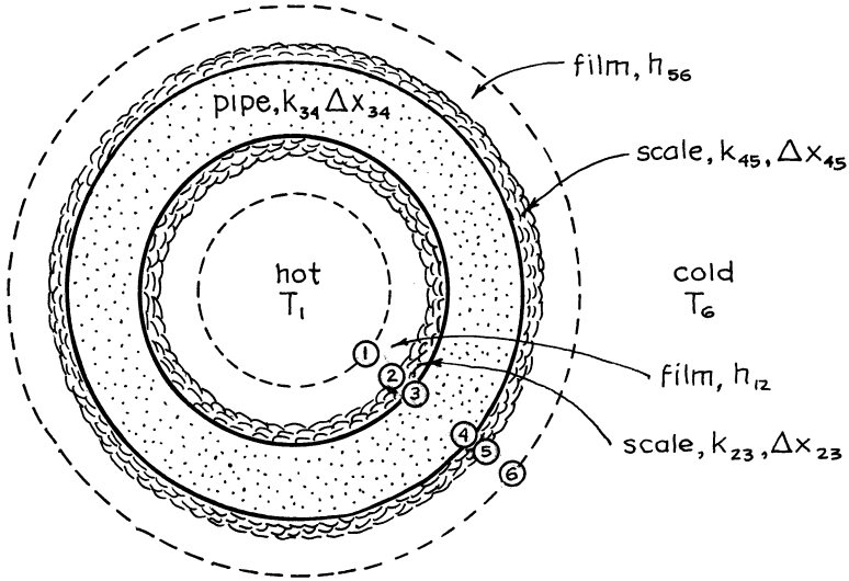
Fig. 10.4 Heat transfer across a scale-coated pipe wall
