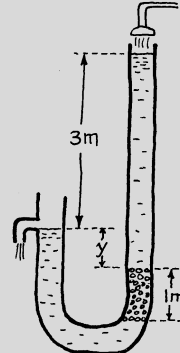
Fig. 6.9 Packed bed below exit in a U tube
