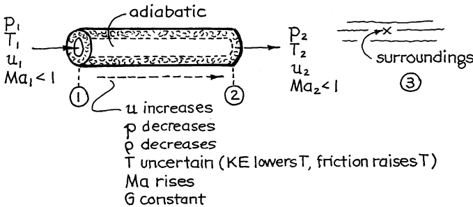
Fig. 3.2 Slow flow in a well-insulated pipe; p_2 = p_3
