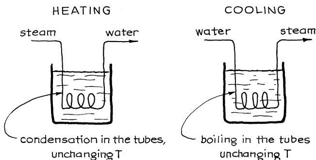
Fig. 13.28 Heating and cooling of a batch of liquid
