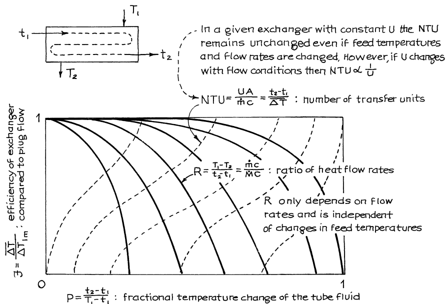
Fig. 13.4 Interrelationship of variables of equations 13.17a and b for shell and tube exchangers. M, C, and T refer to the shell-side fluid; m, c, and t refer to the tube-side fluid; \Delta T = T - t is the temperature driving force
