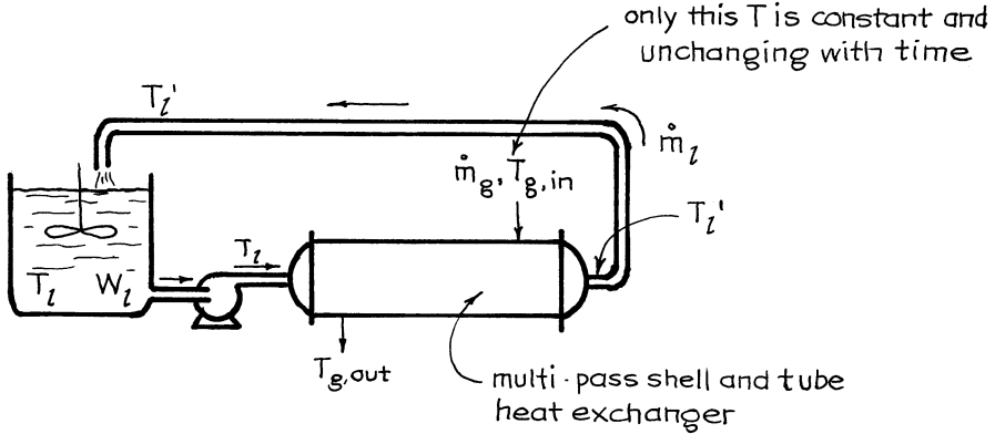
Fig. 13.32 Heating a batch of liquid by means of an external multipass shell and tube exchanger
