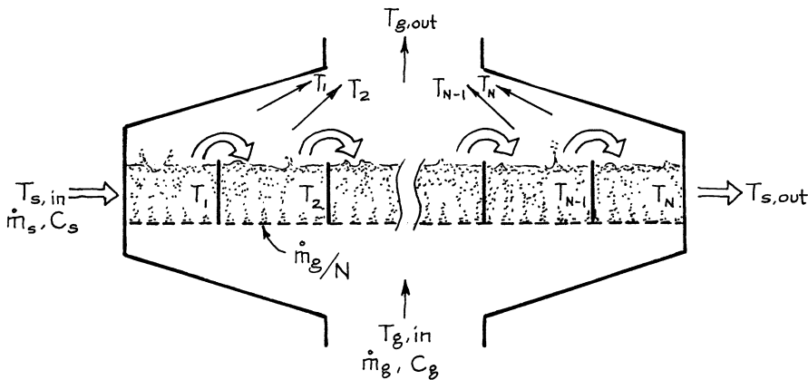
Fig. 14.5 A multistage crossflow fluidized bed heat exchanger
